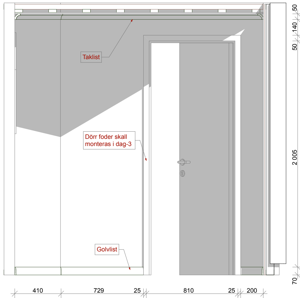
B1 - ELEVATION 1:20
