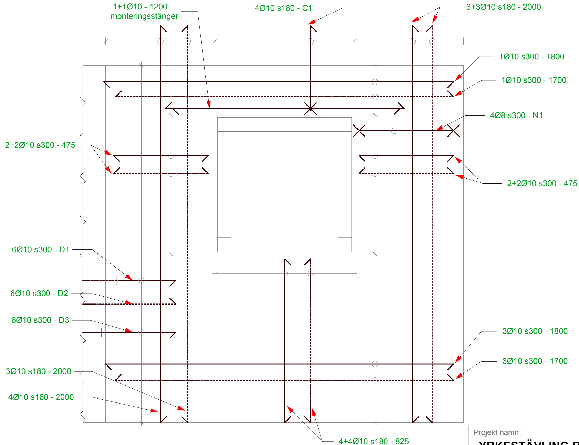
ELEVATION V 1800 ARMERING 2D (2) 1:10
