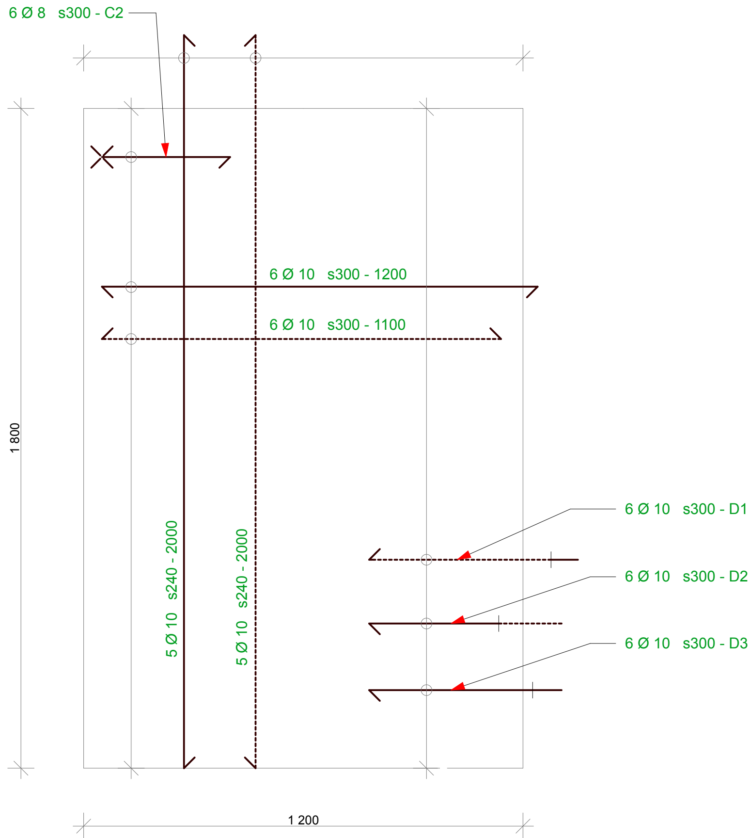
A2 ELEVATION V 1200 ARMERING 2D (1) 1:10
